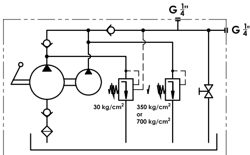
HYDRAULIC SYMBOL
